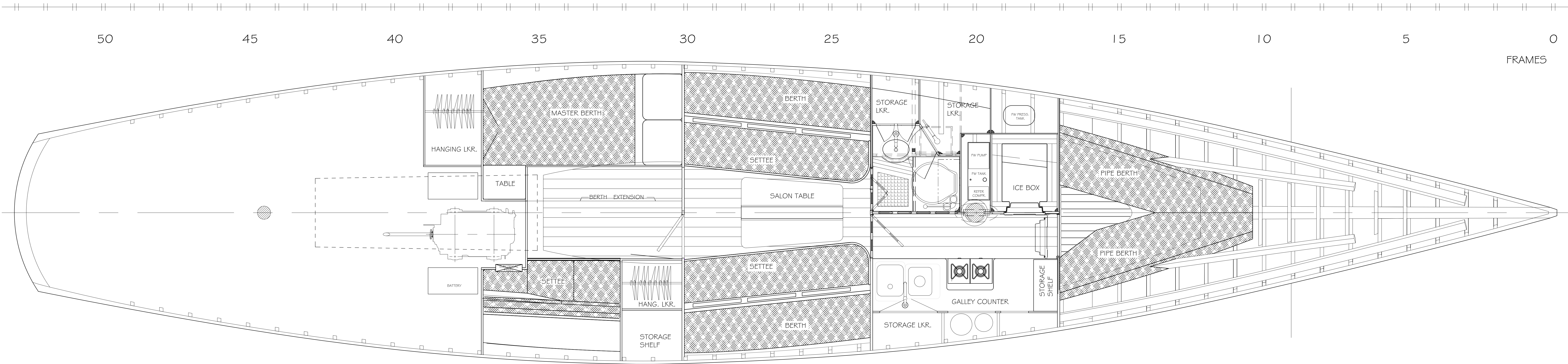
PLAN VIEW
