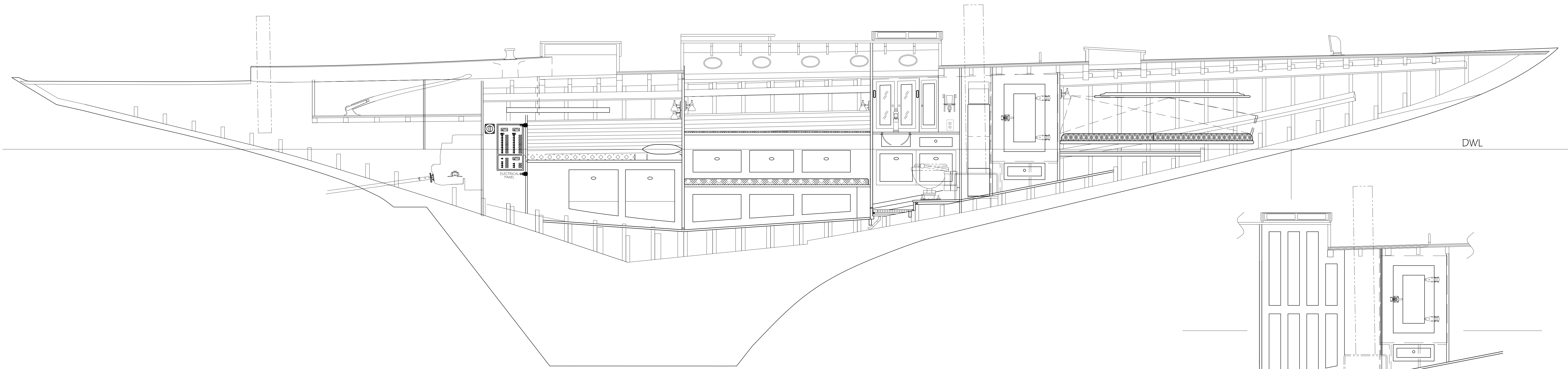
PORT ELEVATION
