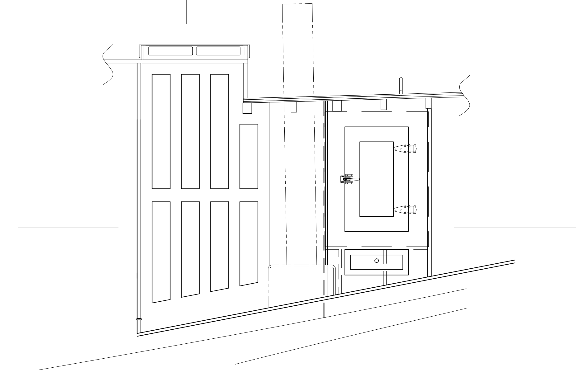
PORT ELEVATION - CENTERLINE GALLEY BLKHD
